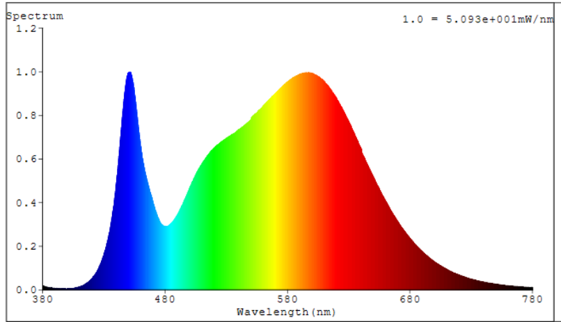
Spectral Distribution
