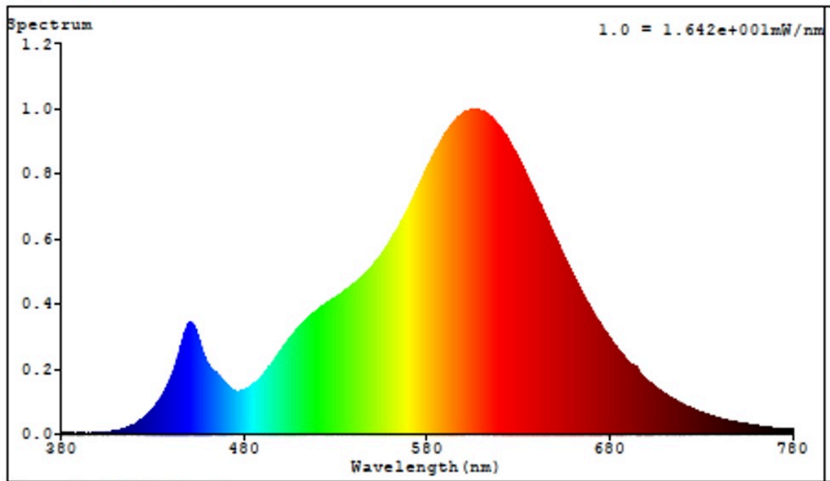
Spectral Distribution
