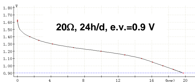
Chart 1. Discharge diagram
